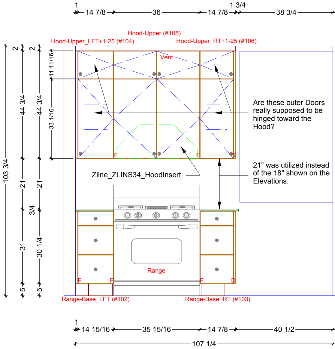
1 KITCHEN ELEVATION - NORTH SCALE: 1/2" = 1' 0"
