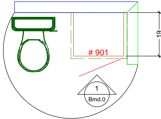
1 BATH-MAID CABINETRY FLOOR PLAN SCALE: 1/2" = 1' 0"
