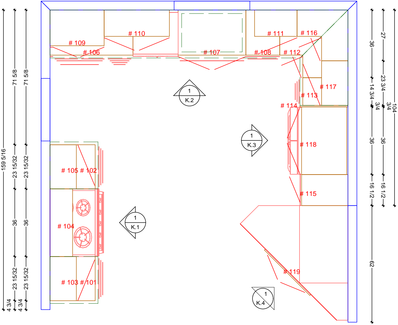
CABINETY FLOOR PLAN SCALE: 3/8" = 1' 0"
