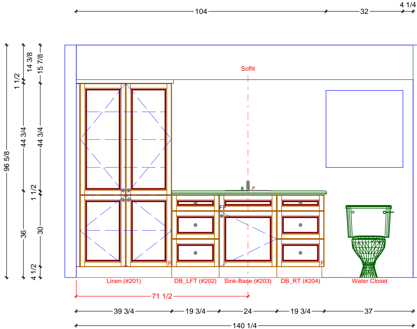
1 MASTER BATH ELEVATION SCALE: 1/2" = 1' 0"
