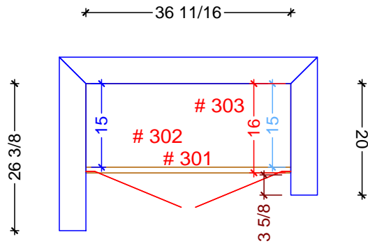
HALL CABINERY FLOOR PLAN SCALE: 1/2" = 1' 0"
