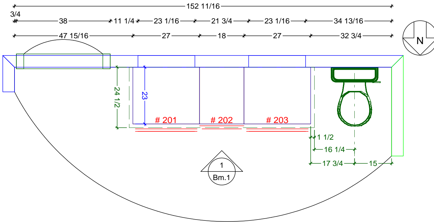
○ MASTER BATH FLOOR PLAN SCALE: 1/2" = 1' 0"
