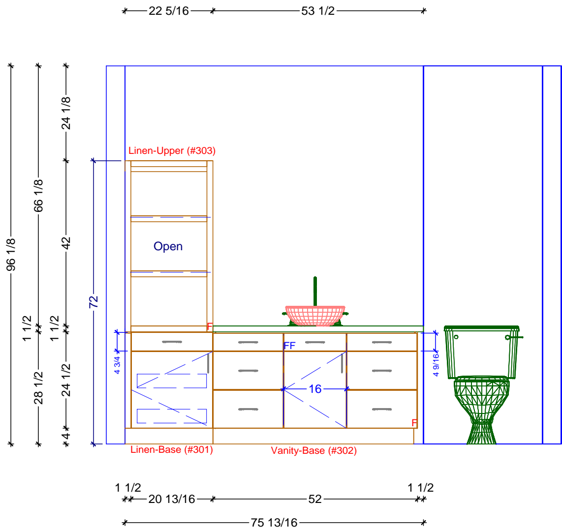
1 HALL BATH ELEVATION - SOUTH SCALE: 1/2" = 1' 0"
