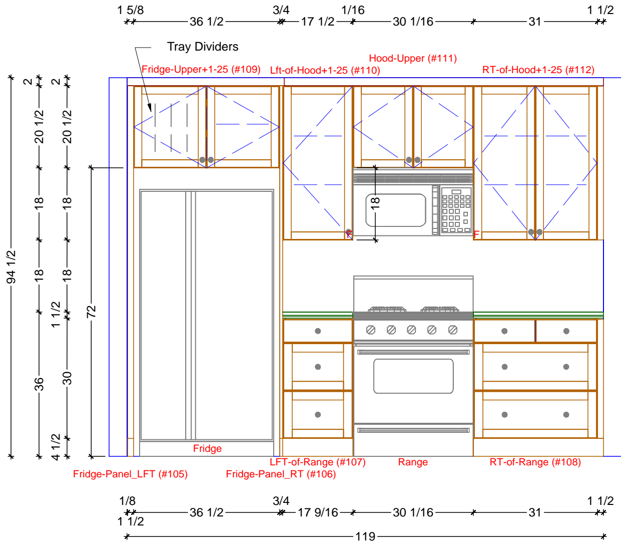
1 KITCHEN ELEVATION - FRIDGE WALL SCALE: 1/2" = 1' 0"
