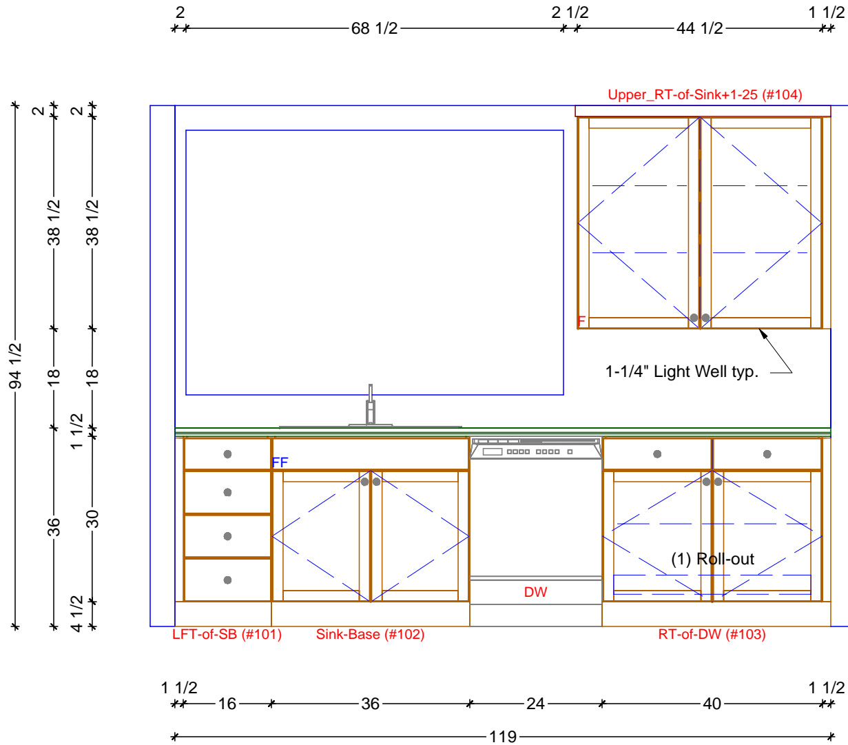
1 KITCHEN ELEVATION - SINK RUN SCALE: 1/2" = 1' 0"
