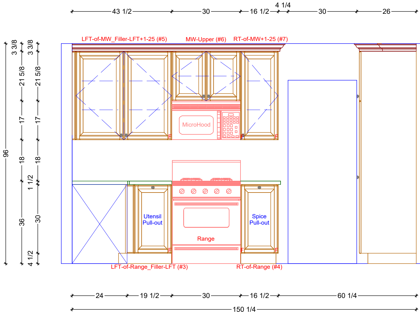
1 KITCHEN ELEVATION - RANGE RUN SCALE: 1/2" = 1' 0"
