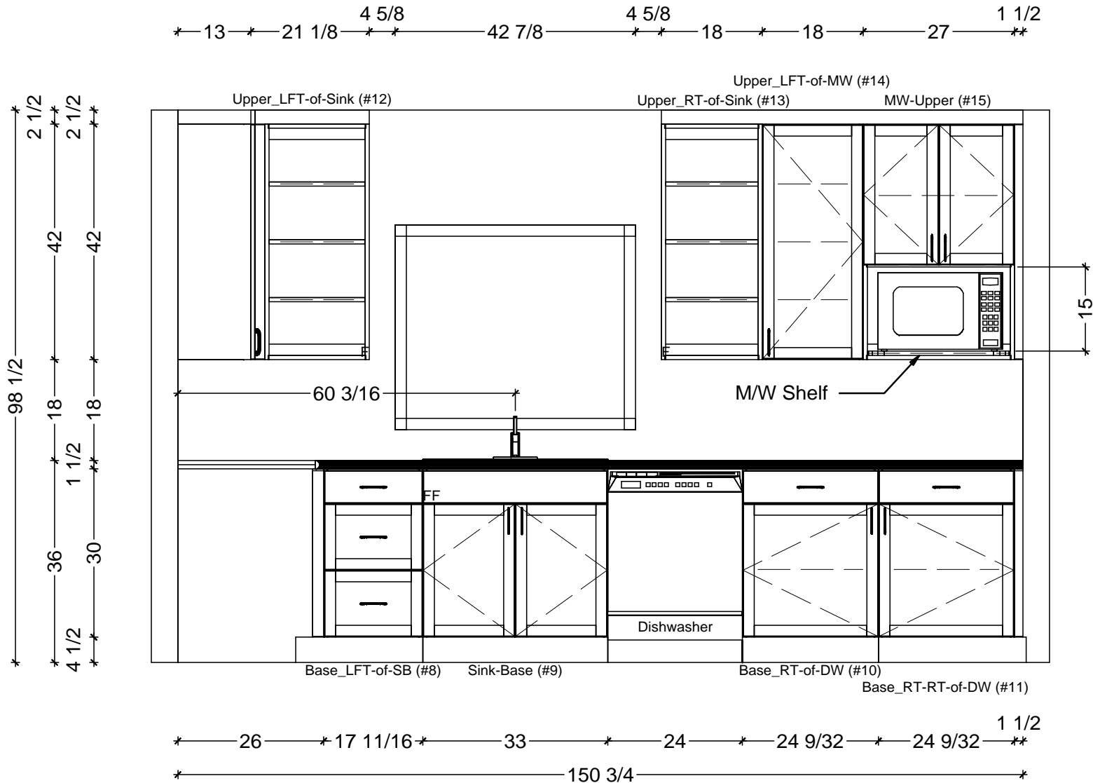
1 KITCHEN ELEVATION - SINK WALL SCALE: 1/2" = 1' 0"
