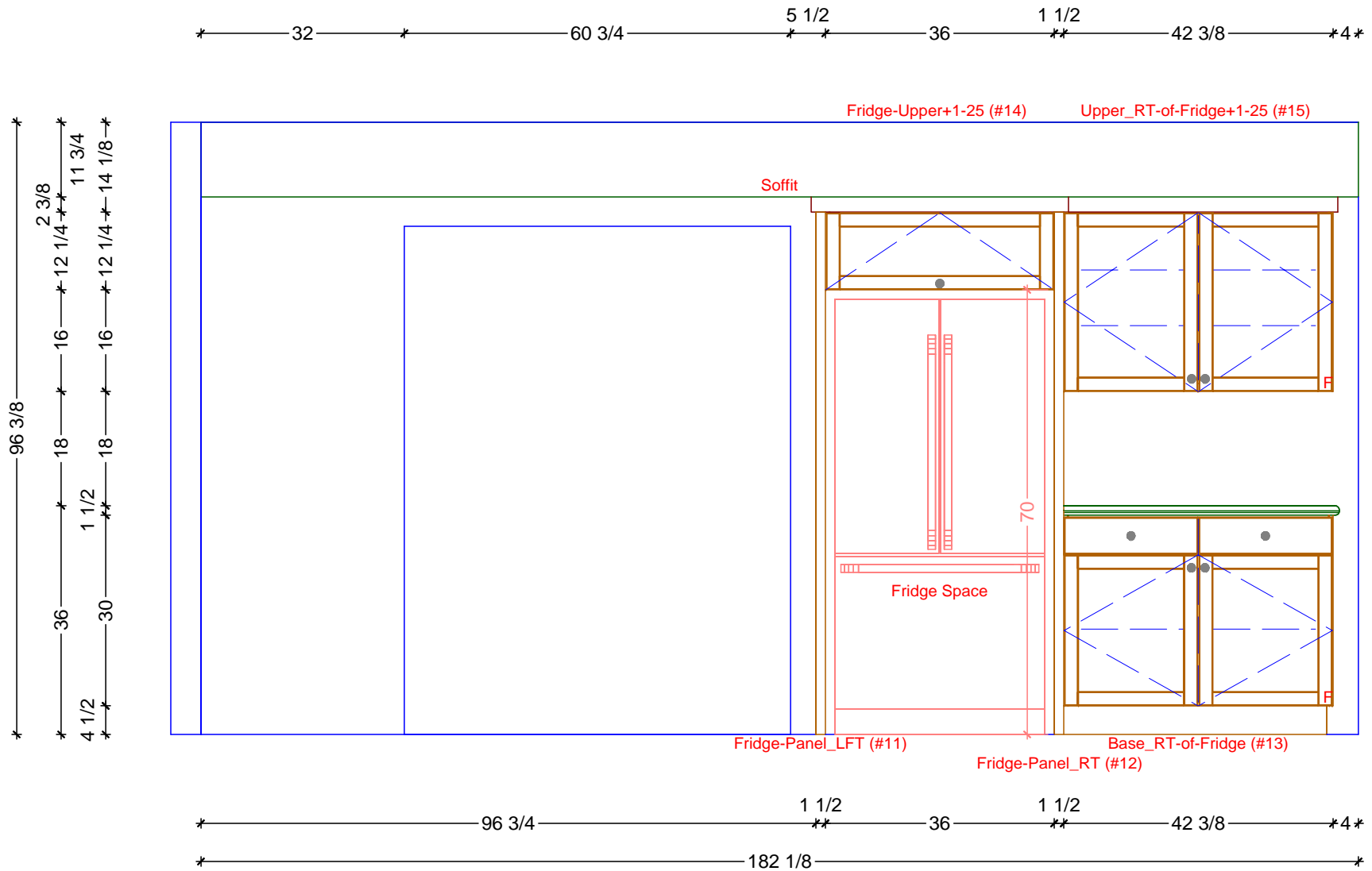
1 KITCHEN ELEVATION - FRIDGE WALL SCALE: 3/8" = 1' 0"
