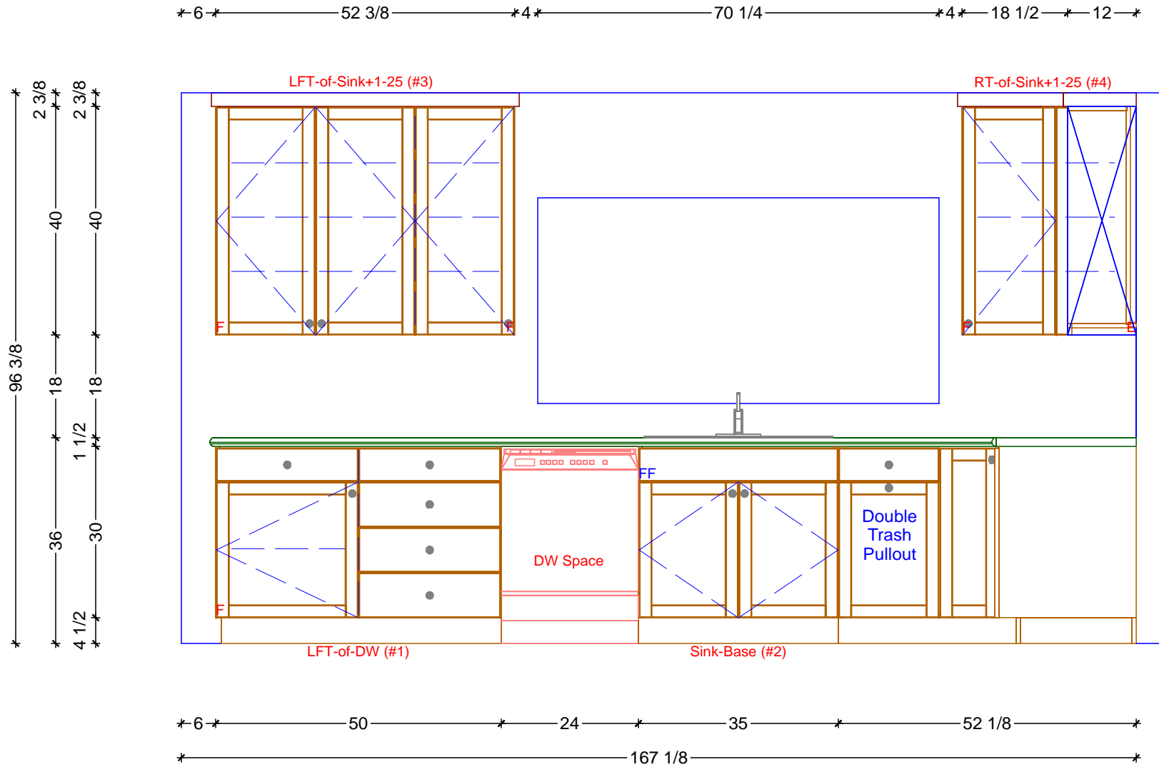
1 KITCHEN ELEVATION - SINK WALL SCALE: 3/8" = 1' 0"
