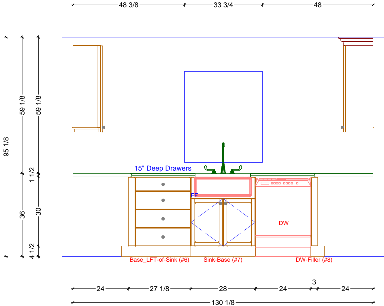
1 KITCHEN ELEVATION - SINK WALL SCALE: 1/2" = 1' 0"
