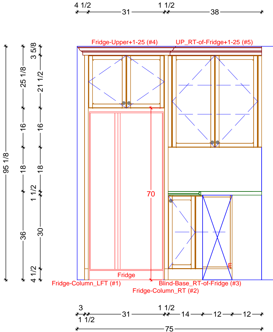
1 KITCHEN ELEVATION - FRIDGE WALL SCALE: 1/2" = 1' 0"
