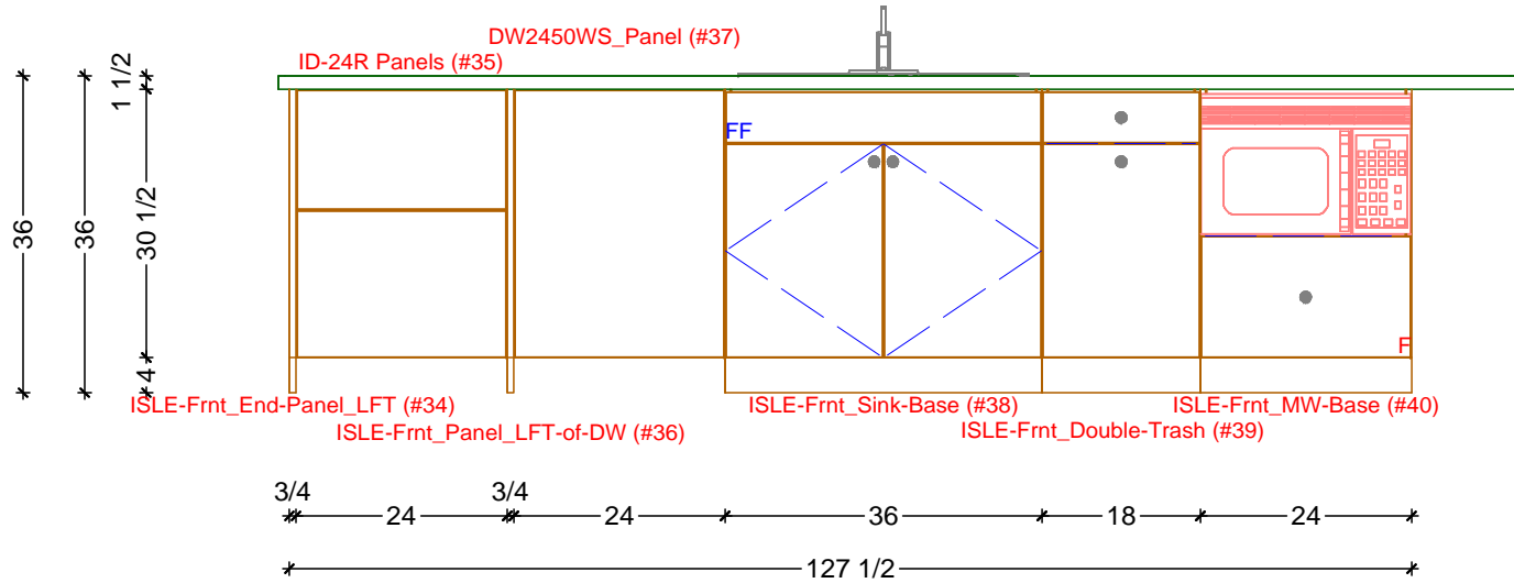
1 KITCHEN ELEVATION - ISLE FRONT SCALE: 1/2" = 1' 0"
