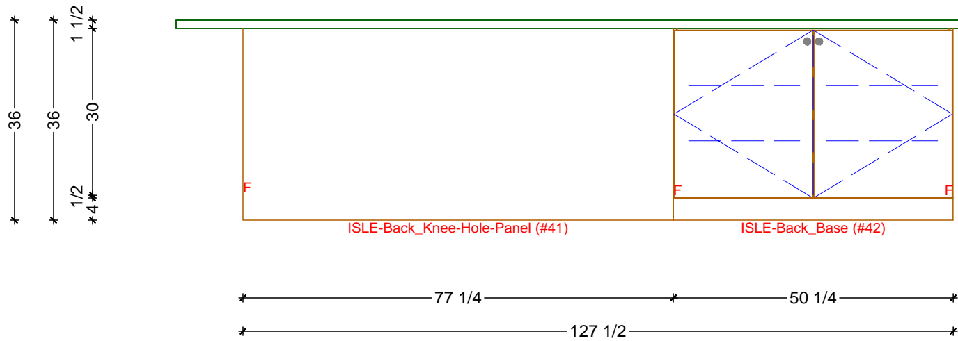
2 KITCHEN ELEVATION - ISLE BACK SCALE: 1/2" = 1' 0"
