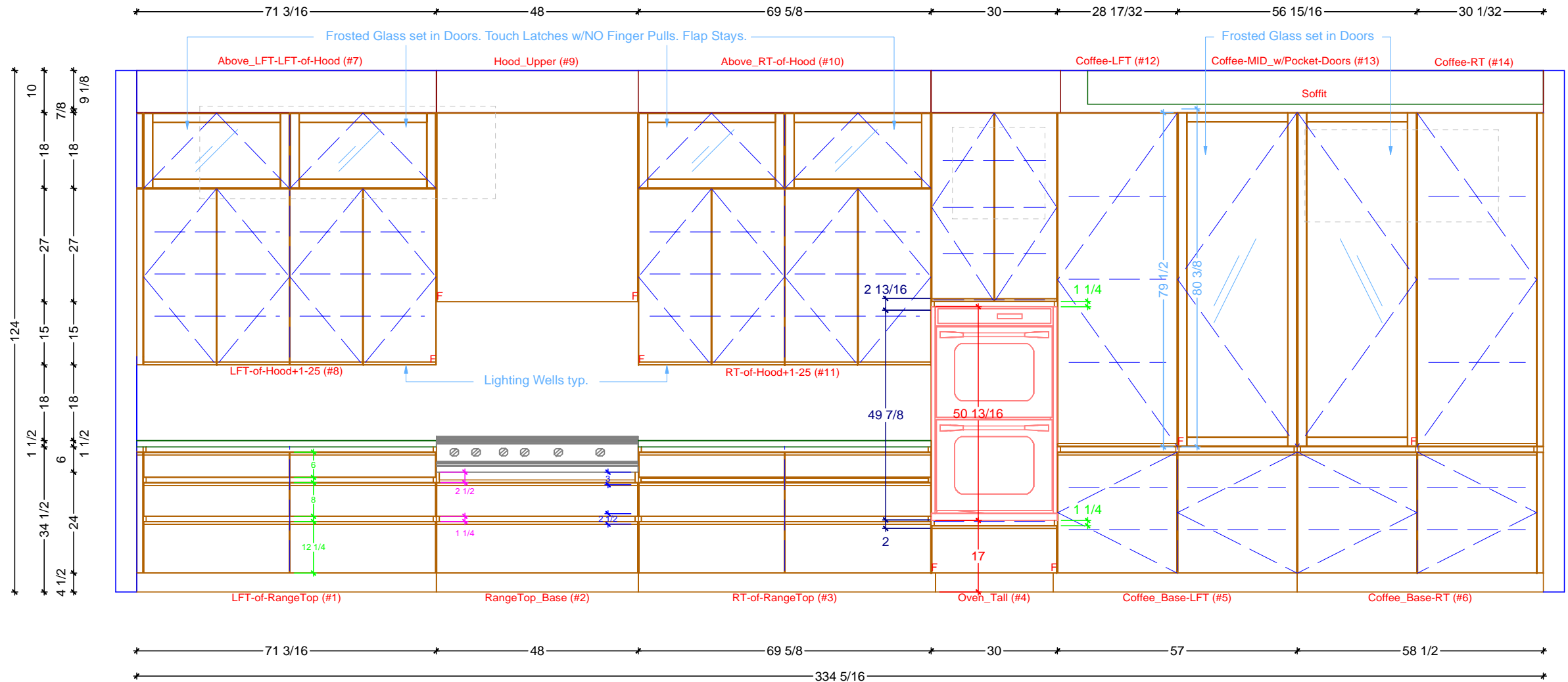
1 KITCHEN ELEVATION - RANGETOP-OVEN-COFFE RUN OF CABINERY SCALE: 1:30
