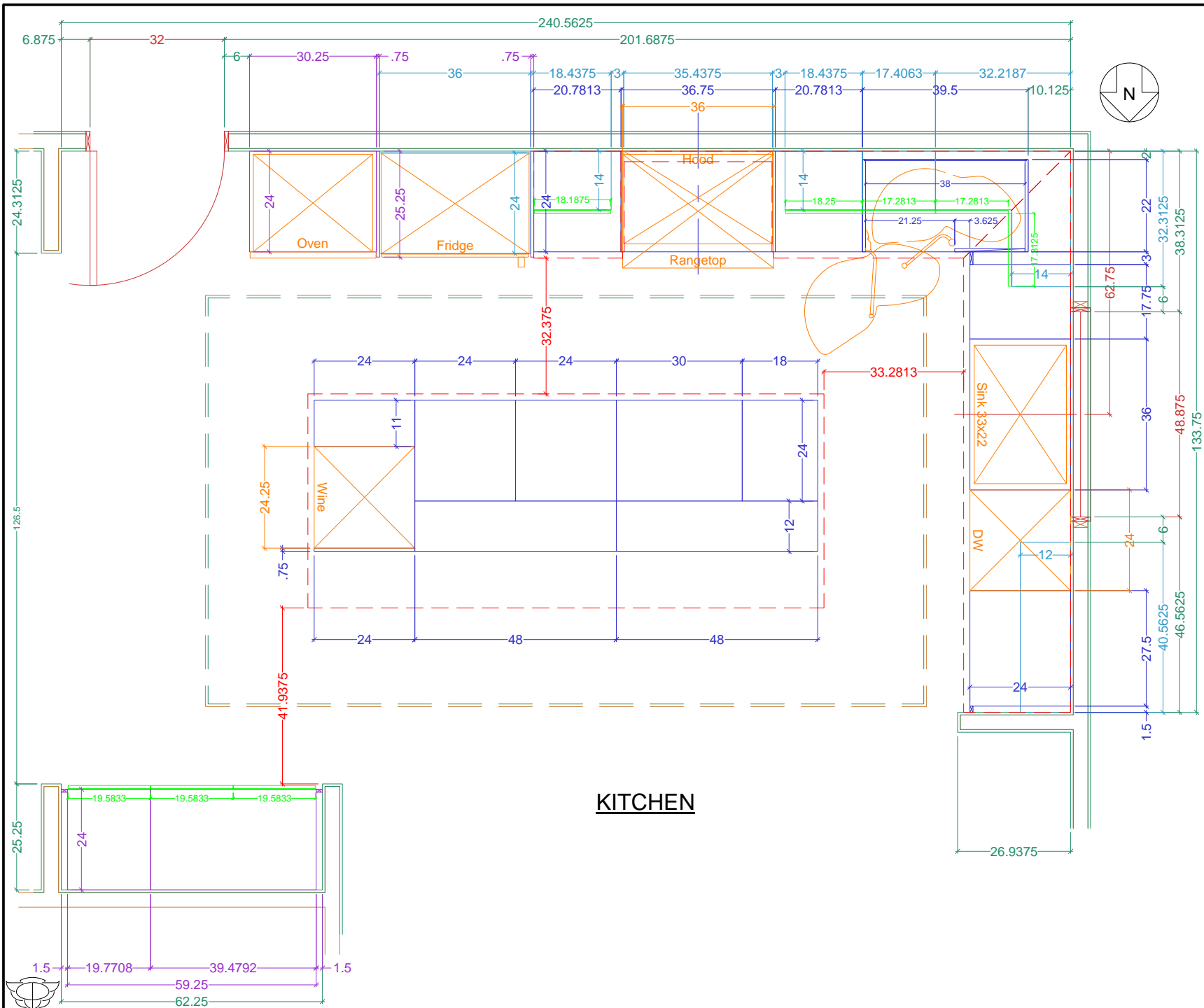
PLAN View -- the Walls
