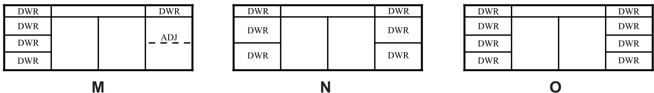
TYPICAL LAY-OUTS FOR 48" THROUGH 72" VANITY CABINETS WITH CENTERED SINKS.
