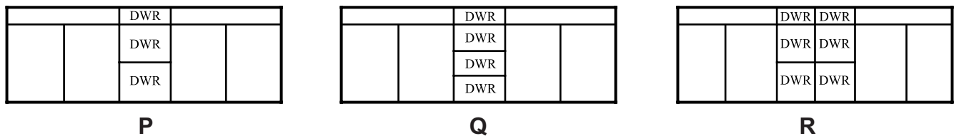
TYPICAL LAY-OUTS FOR 60" THROUGH 84" VANITY CABINETS WITH DOUBLE SINKS.
